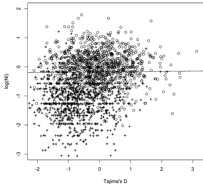
Figure 5. The distribution of values of the logarithm of the neutrality index (NI) and Tajima's D in 1000 simulations under a neutral model (○) and a model involving repeated selective sweeps (+). The parameter values and details of the simulations are described in the main text. The regression line is obtained for neutral data points only and has a slope very close to zero ( -0.0093 ). Notice that almost all points with small values of \log(\text{NI}) and small values of Tajima's D are data points simulated under the selection model.
